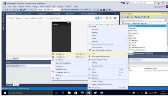
Gambar 10. Activity baru
