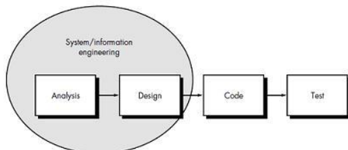
Gambar 1. Model Waterfall
