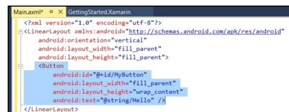
Gambar 6. Source axml
