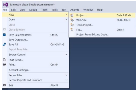
Gambar 3. New Project
